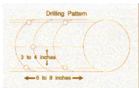
Figure 3. Pattern for drilling holes in logs.
